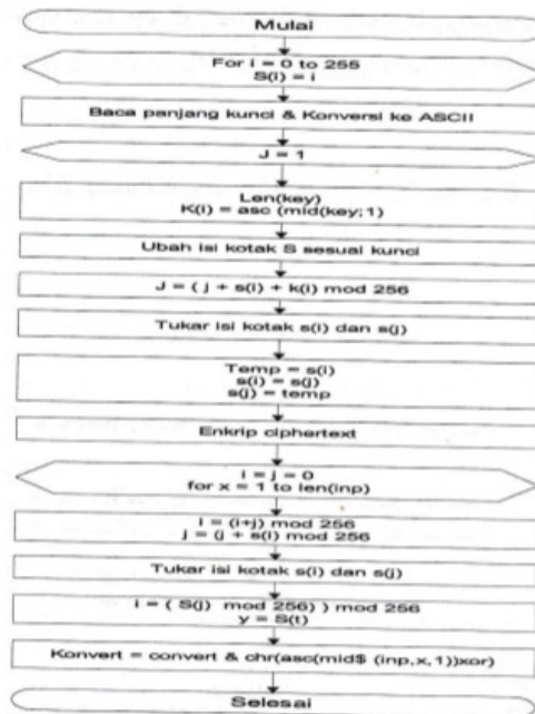
Gambar 6. Diagram Alir Fungsi RC4
