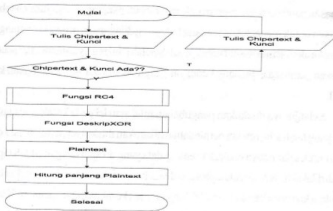
Gambar 5. Diagram Alir Program Deskripsi
